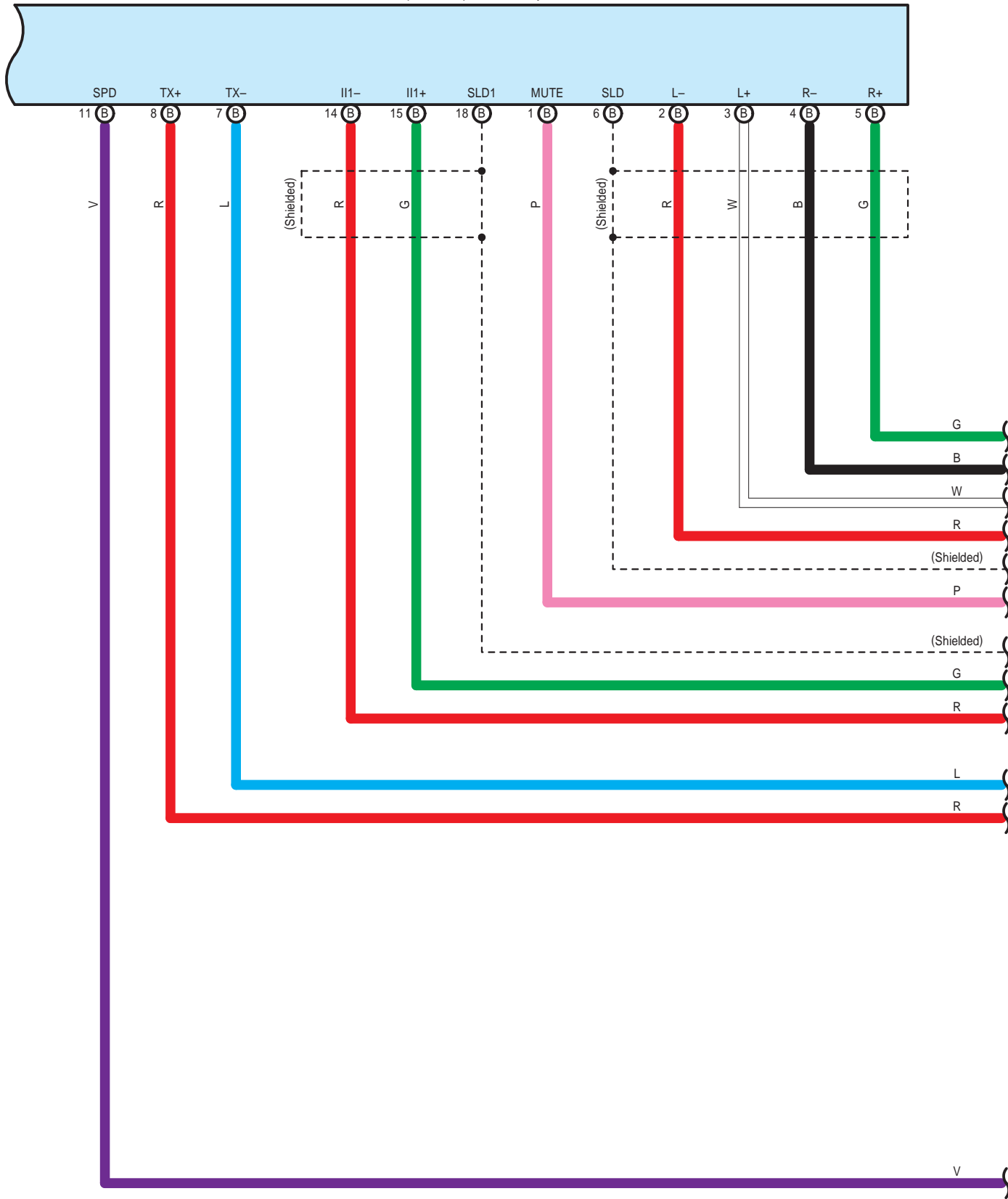
P32(A), P33(B) Stereo Component Amplifier Assembly
