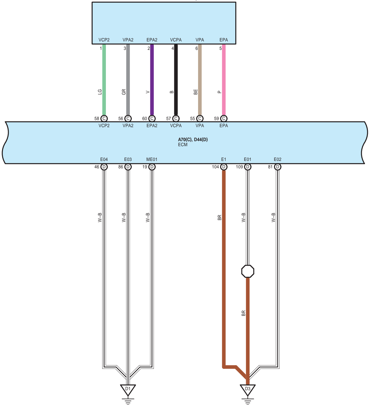
A46 Accelerator Position Sensor (Accelerator Pedal Assembly)
