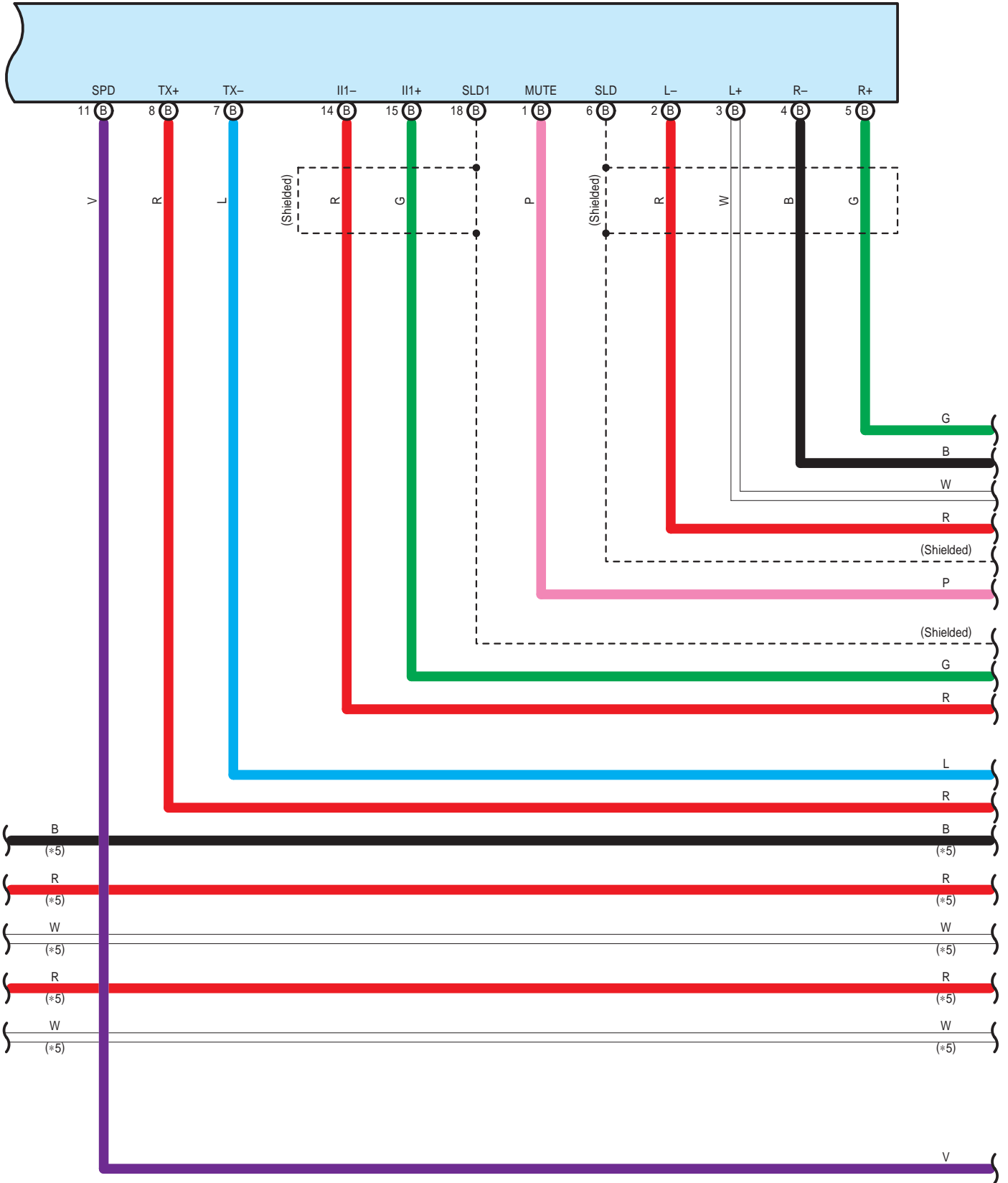
P32(A), P33(B) Stereo Component Amplifier Assembly
