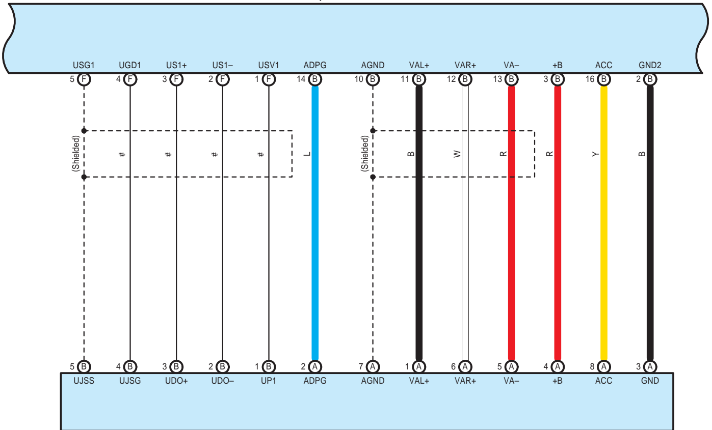
I156(A), I172(B) No. 1 Stereo Jack Adapter Assembly
