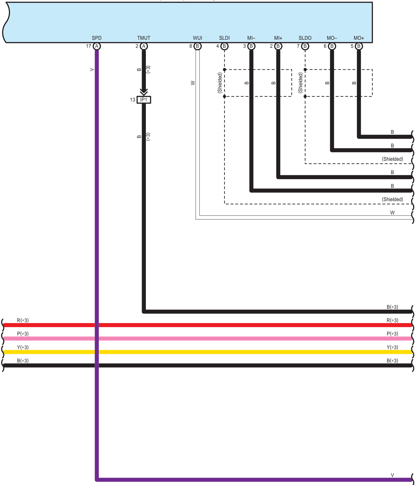
P22(A), P29(B) Stereo Component Amplifier Assembly
