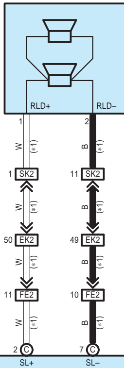
S9 Rear Header Speaker Assembly LH
