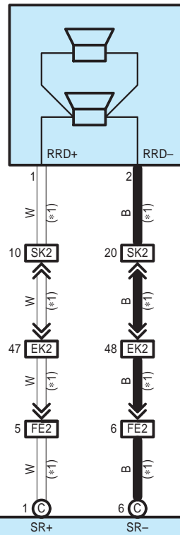
S8 Rear Header Speaker Assembly RH
